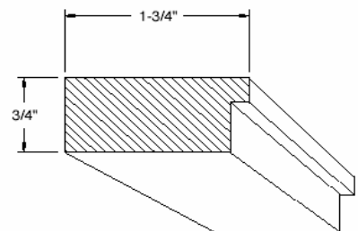
Frieze Mounting Plate 470
