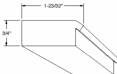
Crown Mounting Plate 384
